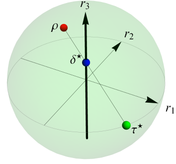
Figure 1. (Color online) Robustness of coherence \mathcal{C}_{\mathcal{R}}(\rho) for a single qubit state \rho = \frac{1}{2}(\mathbb{1} + \vec{r} \cdot \vec{\sigma}) , where \vec{r} is the Bloch vector and \vec{\sigma} is the vector of Pauli matrices. Incoherent states span the thick vertical r_3 axis. The optimization in Eq. (1) is fulfilled by an equatorial pure state \tau^* as depicted, resulting in \mathcal{C}_{\mathcal{R}}(\rho) = (r_1^2 + r_2^2)^{\frac{1}{2}} = 2|\rho_{01}| .
