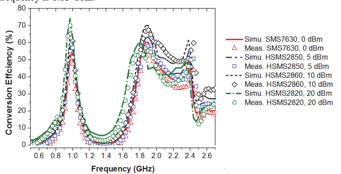
Fig. 17. The simulated and measured conversion efficiency of the rectenna versus frequency for using different types of Schottky diodes at the optimal input power levels. The load resistance is 500 \Omega .
