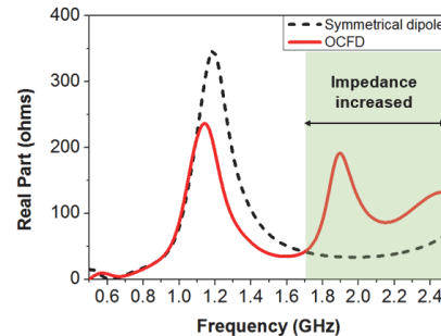
Fig. 5. The simulated real part of the impedance of the symmetrical dipole and the OCFD.
