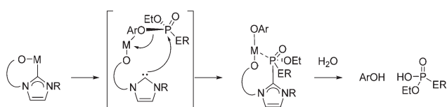
Scheme 8 Proposed mechanism for the destruction of nerve agents with 6-M complexes.
