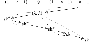
Fig. 7. A strategy on (1 \rightarrow 1) \otimes (1 \rightarrow 1) \rightarrow 1
