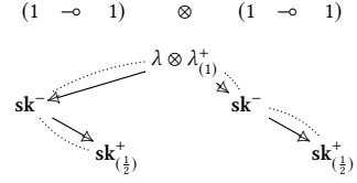
Fig. 10. Non-local probabilistic correlation
