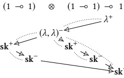
Fig. 17. A parallel strategy
