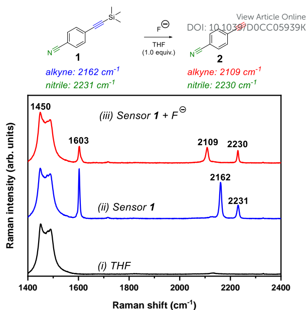
Figure 2 Raman spectral analysis of the desilylation reaction of sensor 1 . Raman spectrum of (i) THF solvent, (ii) Sensor 1 (50 mM) in THF and (iii) Sensor 1 (50 mM) + TBAF (50 mM) in THF (spectrum acquired <1 min after TBAF addition). Spectra were acquired using 785 nm laser excitation for 10 s with a 5× objective lens (~180 mW). The spectra are normalised to the intensity of the peak at 1450 cm -1 . The following peak annotations have been included for clarity: 1450 cm -1 (THF CH 2 def.); 32 1603 cm -1 (C=C phenyl); 2109 cm -1 (C≡C of desilylated compound, 2 ); 2162 cm -1 (C≡C, sensor 1 ) and 2230/2231 cm -1 (C≡N; sensor 1 and compound 2 ).
