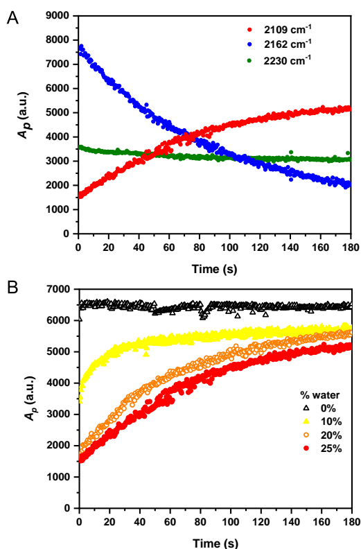
Figure 3 Time-resolved analysis of the desilylation reaction of sensor 1 in aqueous/organic mixtures. A A mixture of sensor 1 (50 mM) and TBAF (75 mM) in THF:water (75:25 v/v) was prepared and Raman spectra were acquired after ~5s following TBAF addition. Raman spectra were acquired continuously using 785 nm laser excitation for 0.5 s using a 5× objective lens (~180 mW) and normalised to the intensity of the THF solvent peak at 1450 cm -1 (CH 2 def.). The peak areas ( A_p ) at 2162 cm -1 (C≡C-TMS), 2109 cm -1 (desilylated alkyne) and 2230-2231 cm -1 (C≡N) are plotted as a function of time. B Analysis of the desilylation of sensor 1 (50 mM) using TBAF (75 mM) as the %water in THF for the reaction mixture is varied (0-25%). A_p is peak area at 2109 cm -1 plotted as a function of time for the different initial % water. Raman spectra were acquired using identical conditions to A .
