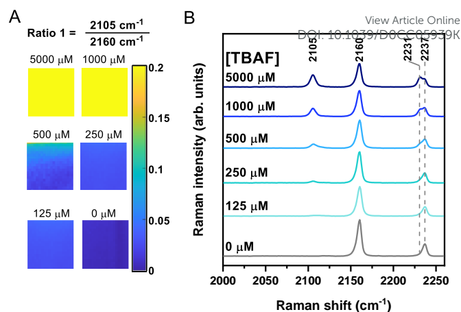
Figure 4 Paper-based detection of fluoride using Raman sensor 1 . A Filter paper was pre-treated with sensor 1 (100 mM in THF, 10 μL) before air-drying and subsequent direct addition of TBAF in THF (300 μL) at the indicated concentrations. Raman maps were acquired across 20 μm × 20 μm (1 μm pixel size; 400 spectra) using 785 nm laser excitation with a 20× objective lens (~180 mW) for 0.5 s. The maps represent the ratio 2105 cm -1 /2160 cm -1 . For the blank sample, 10 mM TBACl replaced TBAF. B Average Raman spectra from maps presented in A . Peak annotations are in cm -1 .
