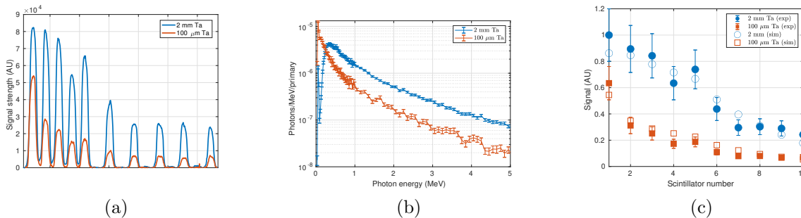
Figure 9. (a) Average brightness across the data from scintillator stack. The ten peaks correspond to the ten scintillators, with the peak on the left corresponding to low energy photons. (b) Expected photon spectra from the experiment generated by Monte Carlo simulations. (c) Comparison of the predicted response of the scintillator stack to the measurement.
