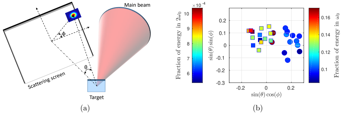
Figure 5. (a) Geometry of the scattering screen monitoring the specular reflection. (b) The fraction of reflected energy on plane of the scattering screen at first (circles) and second harmonic (rectangles) of the laser frequency. The reflected energy of both frequencies are normalized with laser energy and represented by colorbar in the figure.
