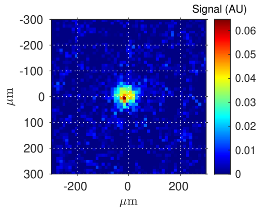
Figure 3. X-ray emission in the range of 0.5 – 2.5 keV measured from the target front surface while shooting a 2 mm thick Ta target.
