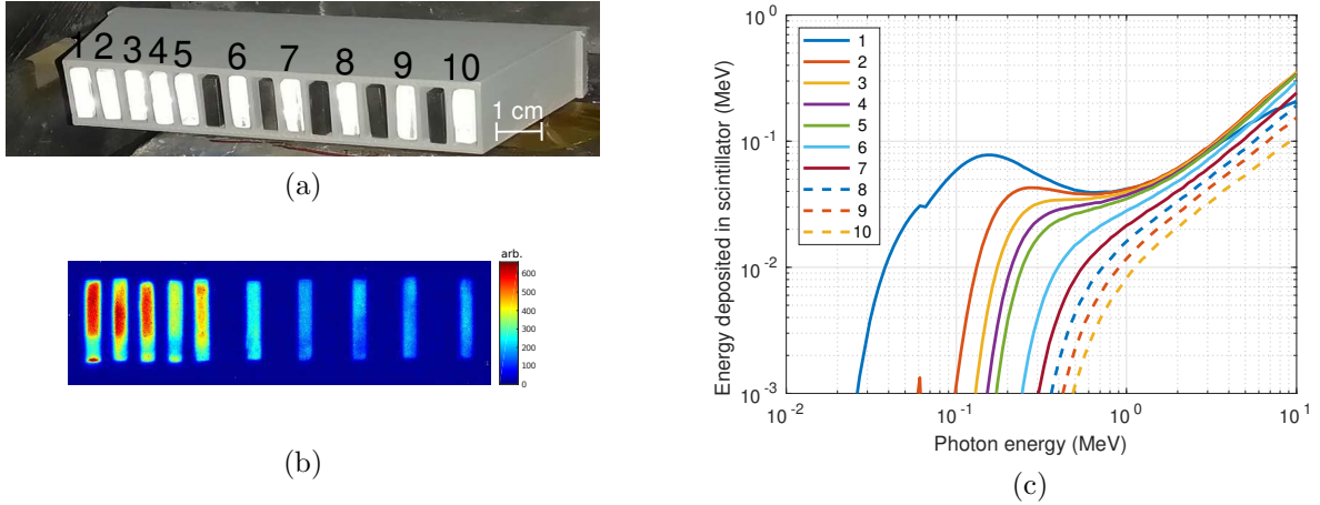
Figure 2. (a) A stack of scintillators and tungsten attenuators placed in a plastic housing and behind a lead collimator. (b) Example of raw data in arbitrary units from imaging the stack of scintillators during a laser shot. (c) Energy deposited in various scintillators in the stack (numbered 1 – 10) as a function of incident photon energy.
