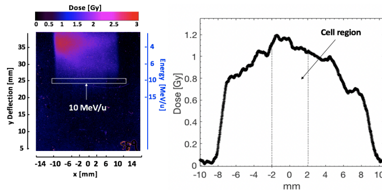
Figure 6. Image of the unlaminated EBT3 irradiated with carbon ions during one shot. The region corresponding to 10 MeV/u carbon ions is also shown (white square) (left). Dose profile along the region highlighted as retrieved by applying the dose calibration. The region where the cells were plated, having a \sim 4 mm width, is also indicated (right).
