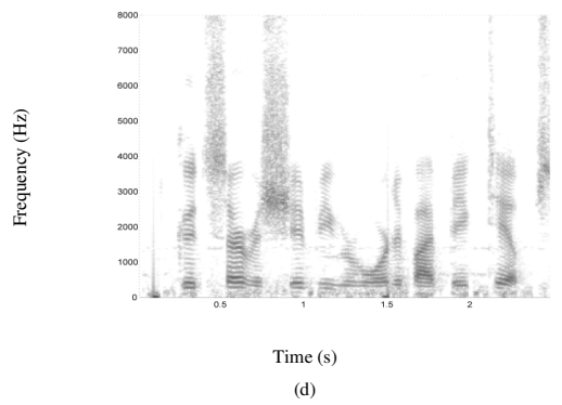
Fig. 6: Comparison of the spectrograms for speech enhanced by both methods in car interior noise at -10 dB. (a) Original clean speech (b) Noisy speech (c) Speech enhanced by OMLSA/IMCRA (d) Speech enhanced by EMDF
