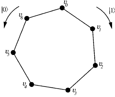
FIG. 2. An example of a cycle graph, with N=7 vertices labeled v_0, v_1 \dots v_6 , and seven edges. Arrows indicate the direction of travel for coin state |0\rangle (anticlockwise) and |1\rangle (clockwise). The cyclic labeling of the vertices does away with the need to label the edges.
