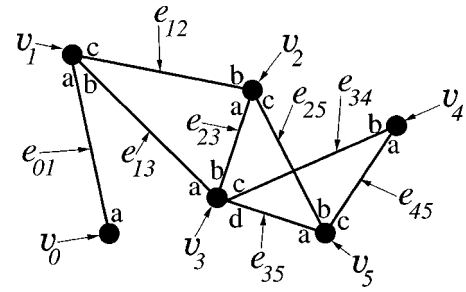
FIG. 1. An example of a general graph, with N=6 vertices labeled v_0, v_1 \dots v_5 , and eight edges labeled e_{01} \dots e_{45} . A labeling of the possible choices of paths from each vertex is given by the letters \{a, b, c, d\} , the degree of this graph being 4.
