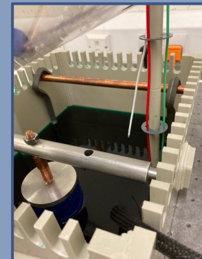
Electrodeposition in Nickel Sulphamate Electrolyte
