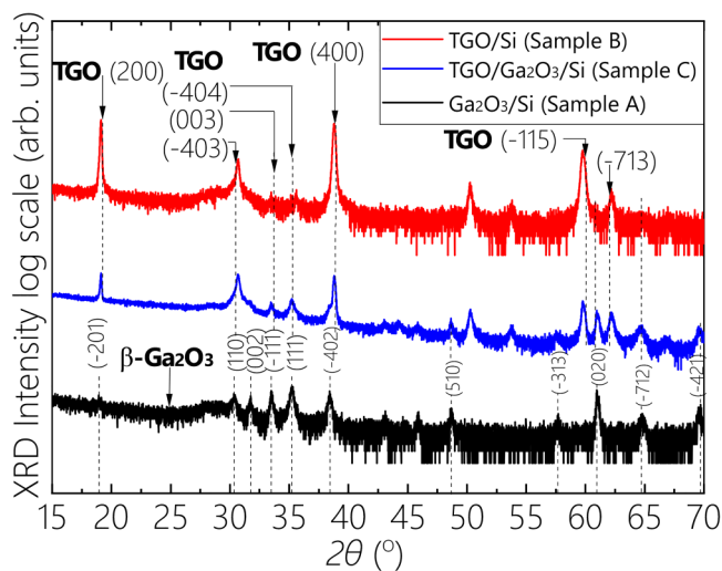
FIG. 3. XRD of polycrystalline \beta - \text{Ga}_2\text{O}_3 and \beta - (\text{Sn}_x\text{Ga}_{1-x})_2\text{O}_3 on Si (111) substrates.
