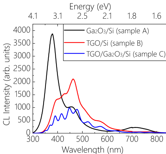
FIG. 4. Room temperature plan view CL spectroscopy for all three samples. Sample C shows the Fabry–Pérot modes from the planar cavity formed by the TGO and \text{Ga}_2\text{O}_3 buffer layer.
