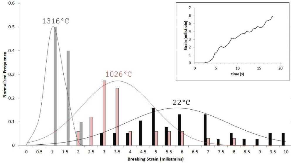
Figure 3. Normalised distribution of breaking strains of fiber splices heated to 1316, 1026 and 22 °C. A typical strain profile measured by the FBG during a splice stress test is shown inset
