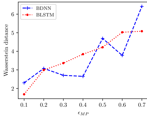
Figure 2: Wasserstein metric of spectral dissimilarity of PSD estimates for the two Bayesian models under a range of missing levels
