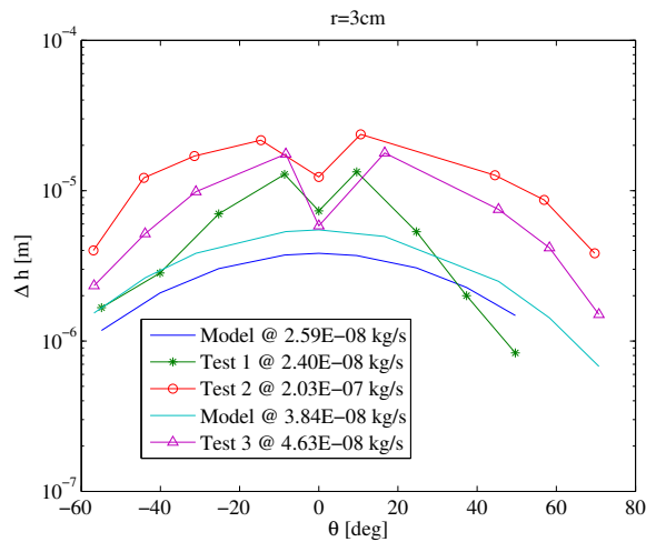
Figure 5. Comparison between the experimental measurements and simulation results for the thickness of the material deposited on the collection plate at 3 cm from the spot.
