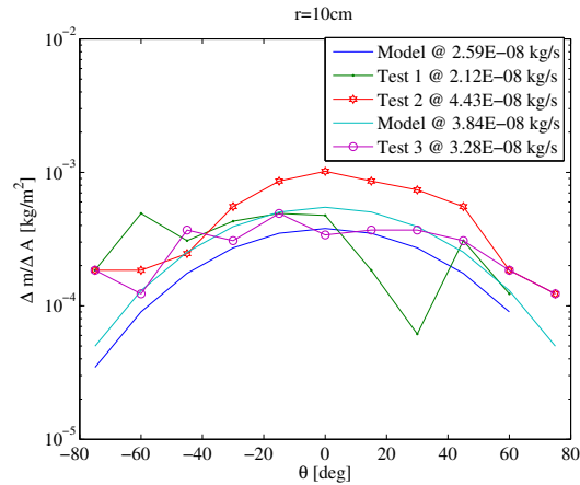
Figure 4. Deposited mass per unit area: experimental result vs. model prediction at 10 cm from the spot.
