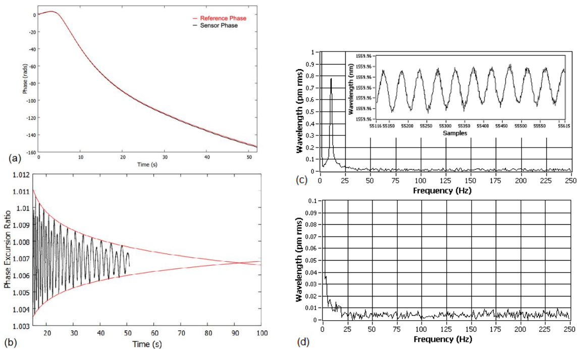
Figure 3. (a) Phase excursions of sensor and reference FBG reflections during OPD tuning (~1% of initial OPD, i.e. 40 \mu\text{m} ). (b) Convergence of sensor wavelength determination process on correct \lambda_s/\lambda_{\text{ref}} ratio of 1.006598. (c) Amplitude spectrum and time plot (inset) of sensor wavelength during small (~5 pm rms) 10 Hz perturbation of cantilever. (d) Spectral noise floor (<10 fm/ \sqrt{\text{Hz}} ) of system recorded using athermal reference FBG.
