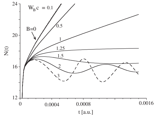
FIG. 1. The final number of created electron-positron pairs as a function of the interaction time for seven different widths of the magnetic field. Parameters used include E = 12.5c^3 , W_E = 0.1/c , and B = 0.6c^3 . B = 0 case is the upper dashed line.
