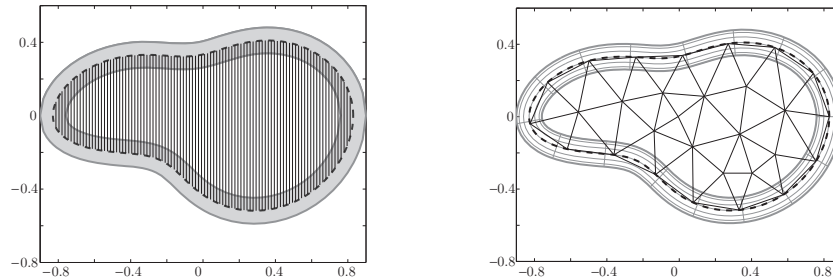
FIGURE 2. Overlapping boundary-layer subdomain \Omega_{[0,2\sigma]} and interior subdomain \Omega_\sigma (left); layer-adapted tensor-product mesh in \Omega_{[0,2\sigma]} and quasiuniform Delaunay triangulation in \Omega_\sigma (right).
