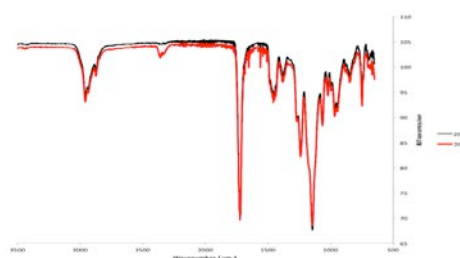
Fig. 2. FTIR spectra for the new foil (2013) and old foil (2012).
