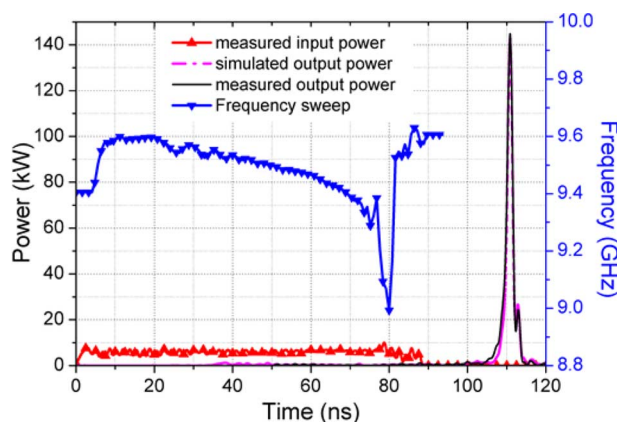
Fig. 8. Measured and simulated microwave outputs from the compression experiment and input microwave waveform and frequency sweep.
