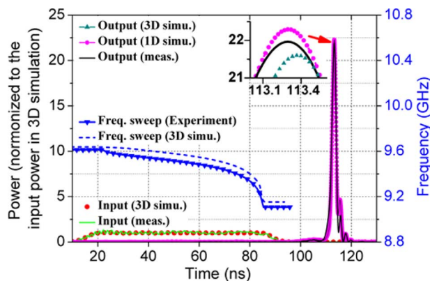
Fig. 7. Simulated and measured compressed pulses. The detail of the compression factors for the different cases are shown in the inset.
