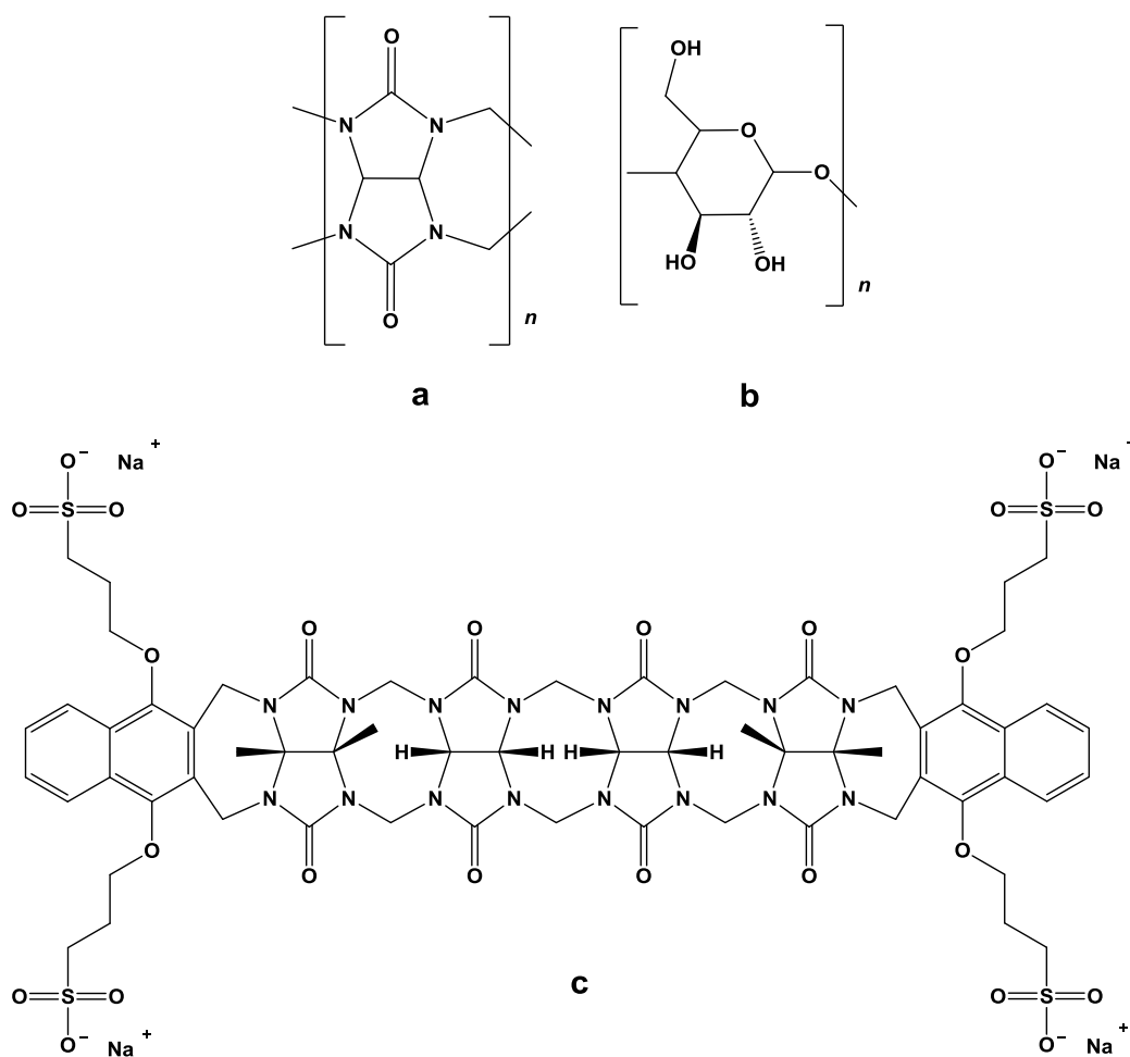
Figure 1. The chemical structures of the macrocycles (a) cucurbit[ n ]uril, (b) n -cyclodextrin, and (c) Motor2.
