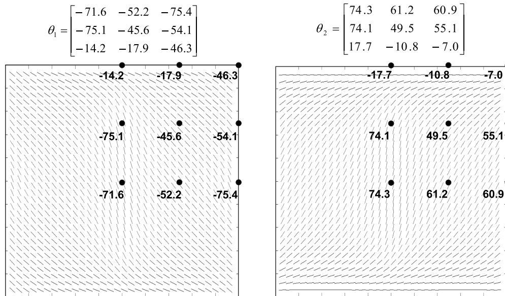
Fig. 10 The optimum nonlinear variation ( 3 \times 3 control points for each layer) of fiber-orientation angles for maximum buckling load of the square simply supported VAT plate design for case A.
