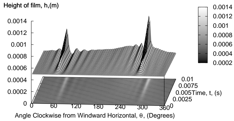
Figure 23: Numerical prediction of temporal evolution in real time of film height under full loading conditions.
