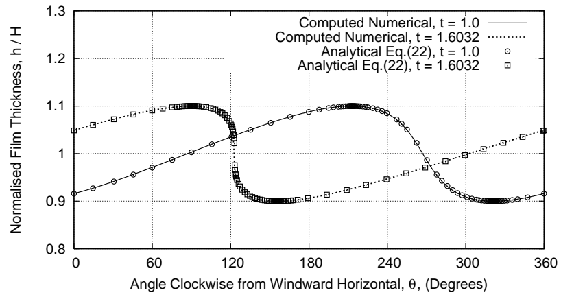
Figure 7: Comparison of analytical solution for constant shear (22) with computed numerical results for spatial distribution of normalised film height on cylinder at t = 1 s and t = 1.6032 s.
