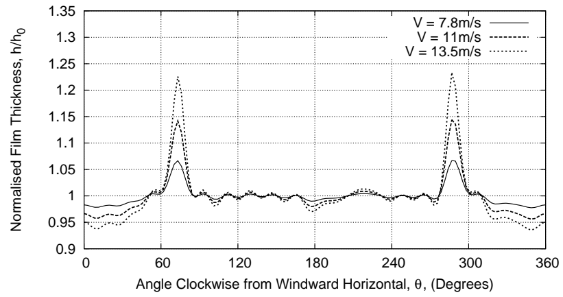
Figure 15: Effect of varying shear-loading value T through variation of the incident wind speed V with constant distribution of C_F on variation of normalised film height with angle from windward horizontal at t = 6.9 \times 10^{-3} s.
