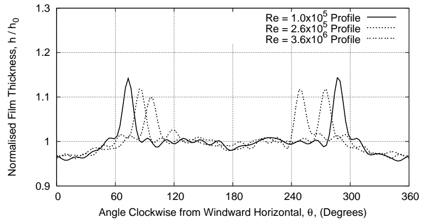
Figure 21: Effect of varying Reynolds number through change of flow regime on the variation of normalised film height with angle from windward horizontal at t = 6.9 \times 10^{-3} s, for shear and surface-tension loading.
