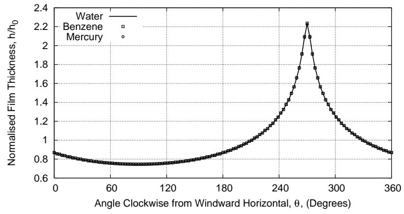
Figure 11: Comparison of normalised film heights of water, benzene and mercury as functions of angle \theta at reduced time \tau = 0.4 .
