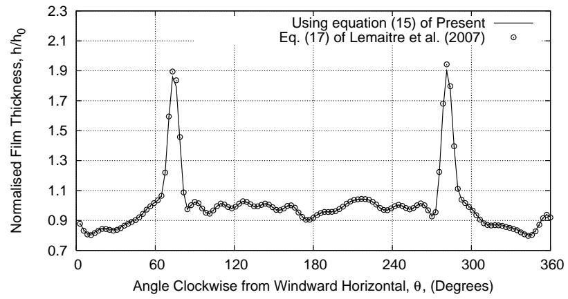
Figure 14: Comparison of normalised film height under the effects of shear and surface tension from present numerical solver for evolution equation (15) and equation (17) of Lemaitre et al. [11], using identical C_F distribution, at t = 34.0 \times 10^{-3} s .
