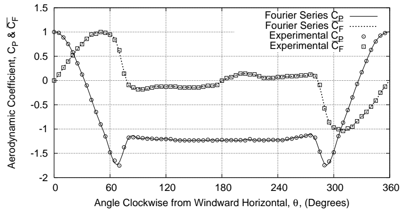
Figure 3: Aerodynamic coefficients C_P and C_F used in the numerical calculations and those measured experimentally by Achenbach [1] at Re = 1 \times 10^5 .
