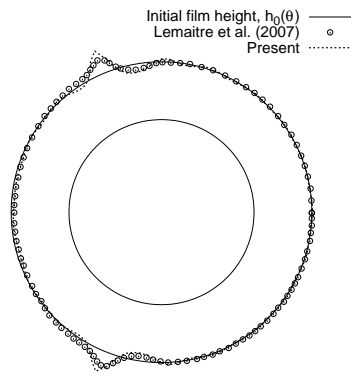
Figure 18: Comparison of present numerical results with result of Lemaitre et al. [11] for variation of film height (100×actual) at t = 6.9 \times 10^{-3} s , under the effects of pressure and surface tension, where the incident wind acts from the left.
