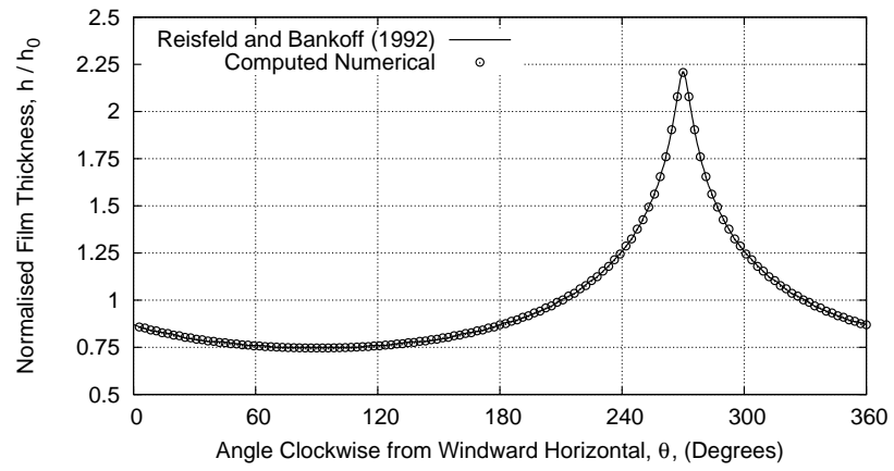
Figure 6: Comparison of the analytical solution of Reisfeld and Bankoff [16] given in (17) – (20) with computed numerical results for normalised film height on cylinder at Bo = 1.4 \times 10^7 : spatial distribution ( 0 \leq \theta \leq 360^\circ ) at \tau = 0.4 .
