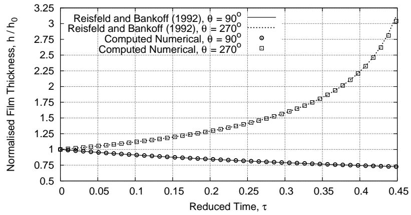
Figure 5: Comparison of the analytical solution of Reisfeld and Bankoff [16] given in (17) – (20) with computed numerical results for normalised film height on cylinder at Bo = 1.4 \times 10^7 : temporal evolution at top ( \theta = 90^\circ ) and bottom ( \theta = 270^\circ ) of the cylinder.
