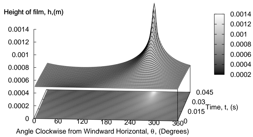
Figure 9: Numerical prediction of temporal evolution of the film height in real time, under gravity and surface-tension effects only.
