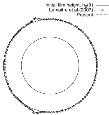
Figure 13: Comparison of present numerical results with the results of Lemaitre et al. [11] for variation of film height ( 100 \times actual) at t = 6.9 \times 10^{-3} s , under the effects of shear and surface tension, where the incident wind acts from the left.
