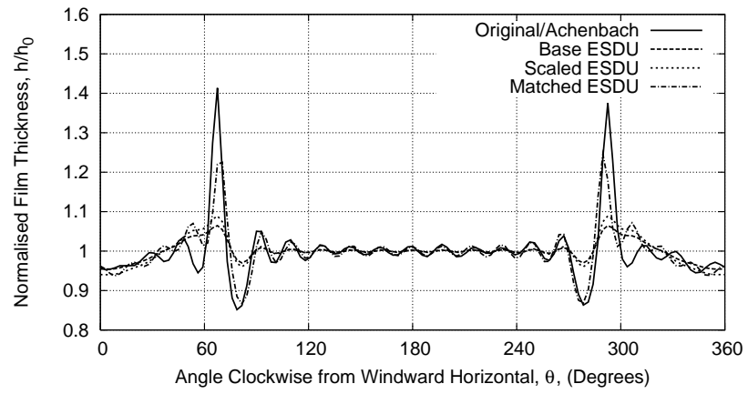
Figure 20: Comparison of the effect that various distributions of C_P have on the normalised film height profile, at t = 6.9 \times 10^{-3} s, under pressure and surface-tension loading.
