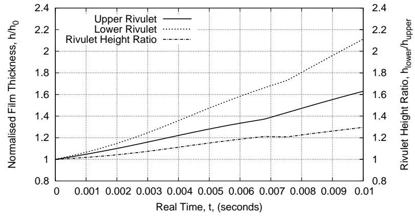
Figure 24: Early temporal evolution of normalised film height of upper and lower rivulets and ratio between these.
