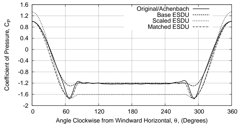
Figure 19: Profiles of the four distributions of C_p used, namely that used by Achenbach [1], base ESDU, scaled ESDU and matched ESDU.
