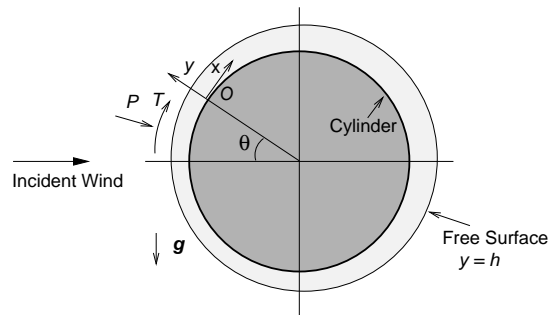
Figure 1: A thin fluid film on a horizontal cylinder.
