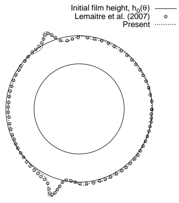
Figure 25: Comparison of present numerical results with result of Lemaitre et al. [11] for variation of film height (100×actual) at t = 6.9 \times 10^{-3} s under full loading conditions, where the incident wind acts from the left.
