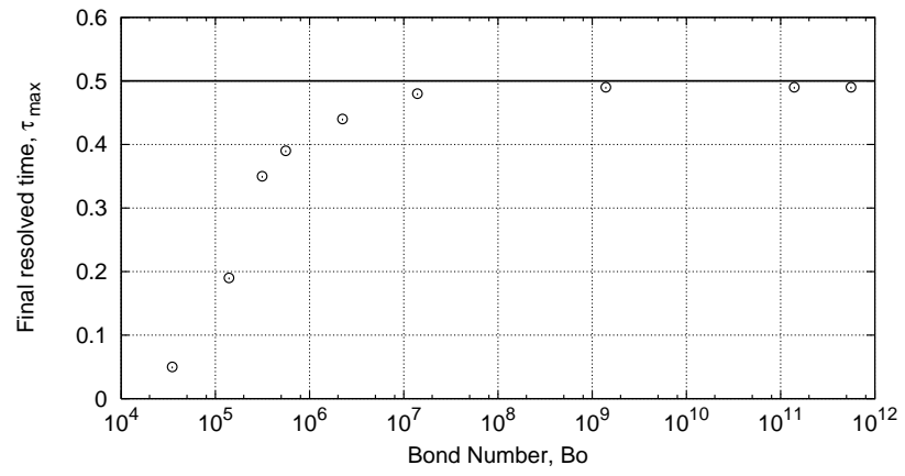
Figure 4: Final resolved time, \tau_{max} as a function of Bo.
