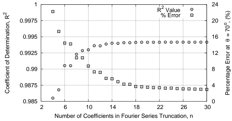
Figure 2: Variation of the coefficient of determination R^2 and percentage error at \theta = 70^\circ with the number of terms, n , in the truncated Fourier series representation of the pressure coefficient C_P .
