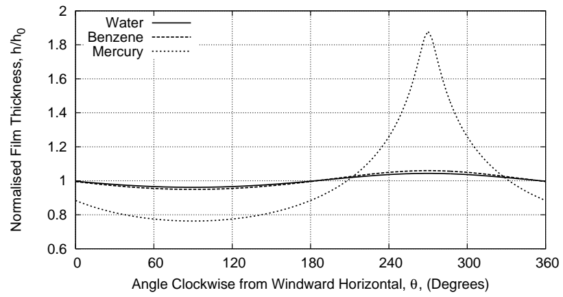
Figure 10: Comparison of normalised film heights of water, benzene and mercury as functions of angle \theta at real time t = 0.4 \times 10^{-3} s.
