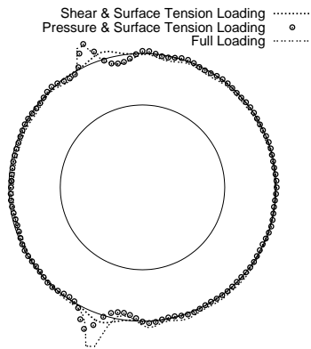
Figure 26: Comparison of present numerical results under three loading conditions for variation of film height ( 100\times actual) at t = 6.9 \times 10^{-3} s , where the incident wind acts from the left.
