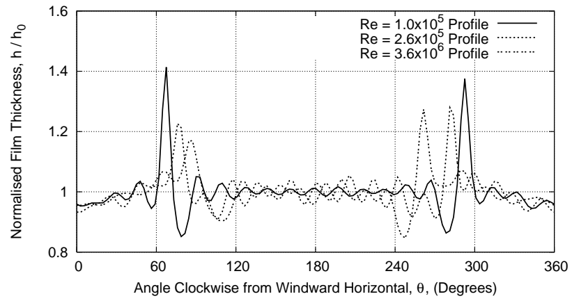
Figure 22: Effect of varying Reynolds number through change of flow regime on the variation of normalised film height with angle from windward horizontal at t = 6.9 \times 10^{-3} s, for pressure and surface-tension loading.
