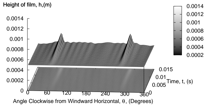
Figure 12: Numerical prediction of the temporal evolution of film height in real time, under shear and surface-tension effects only.
