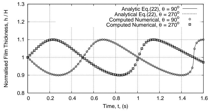
Figure 8: Comparison of analytical solution for constant shear (22) with computed numerical results for normalised film height for temporal evolution at top ( \theta = 90^\circ ) and bottom ( \theta = 270^\circ ) of the cylinder.
