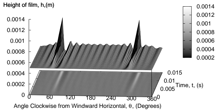
Figure 16: Numerical prediction of the temporal evolution of film height in real time, under pressure and surface-tension effects only.
