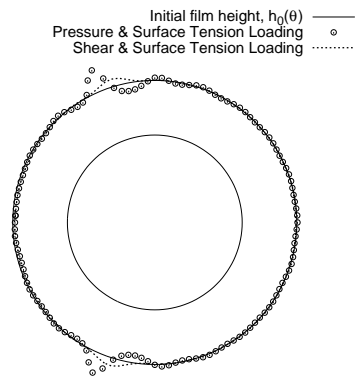
Figure 17: Comparison of film height (100× actual) of present results under shear and surface-tension loading with those under pressure and surface-tension loading at t = 6.9 \times 10^{-3} s, where the incident wind acts from the left.
