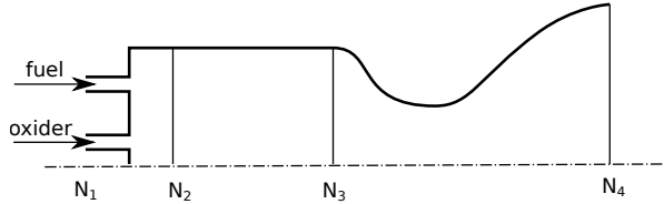
Figure 2. Definition of stations for the rocket injection module (as implemented in a typical rocket engine model).
