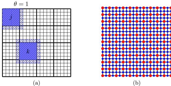
Figure 1: (a) Additive Schwarz subdomains on the boundary ( j ) and in the interior ( k ). The overlapping domain is shown with diagonal lines and the non-overlapping domain is shaded. The overlap is \theta = 1 because the overlapping domain is obtained from the non-overlapping domain by extending by one node in each direction. (b) Coarse and fine grid points with coarse grid points denoted by larger red circles.
