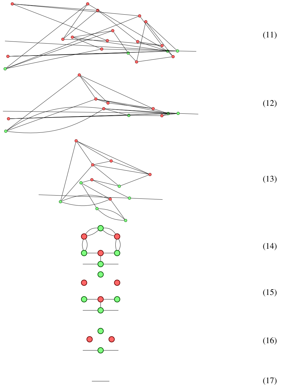
Figure 11: Rewrite sequence 2(b)
