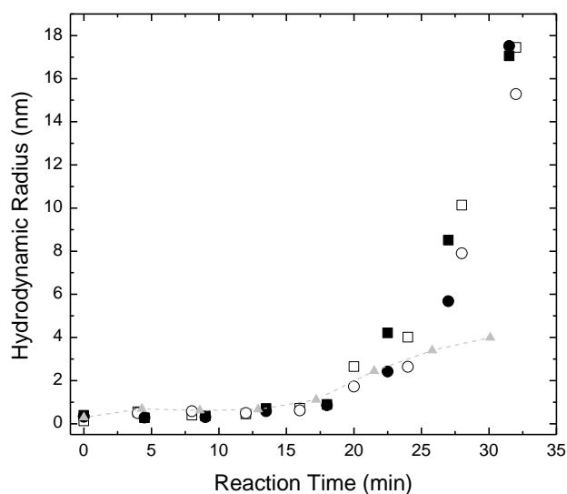
Figure 2. Mean hydrodynamic radii as determined from DLS autocorrelation functions for \text{CaCO}_3 at (□) R/C 100 and (■) R/C 200, and \text{BaCO}_3 at (○) R/C 100 and (●) R/C 200. Data for \text{Na}_2\text{CO}_3 at (▲) R/C 200 is included for comparison, with further comparative data included in the S.I. 8
