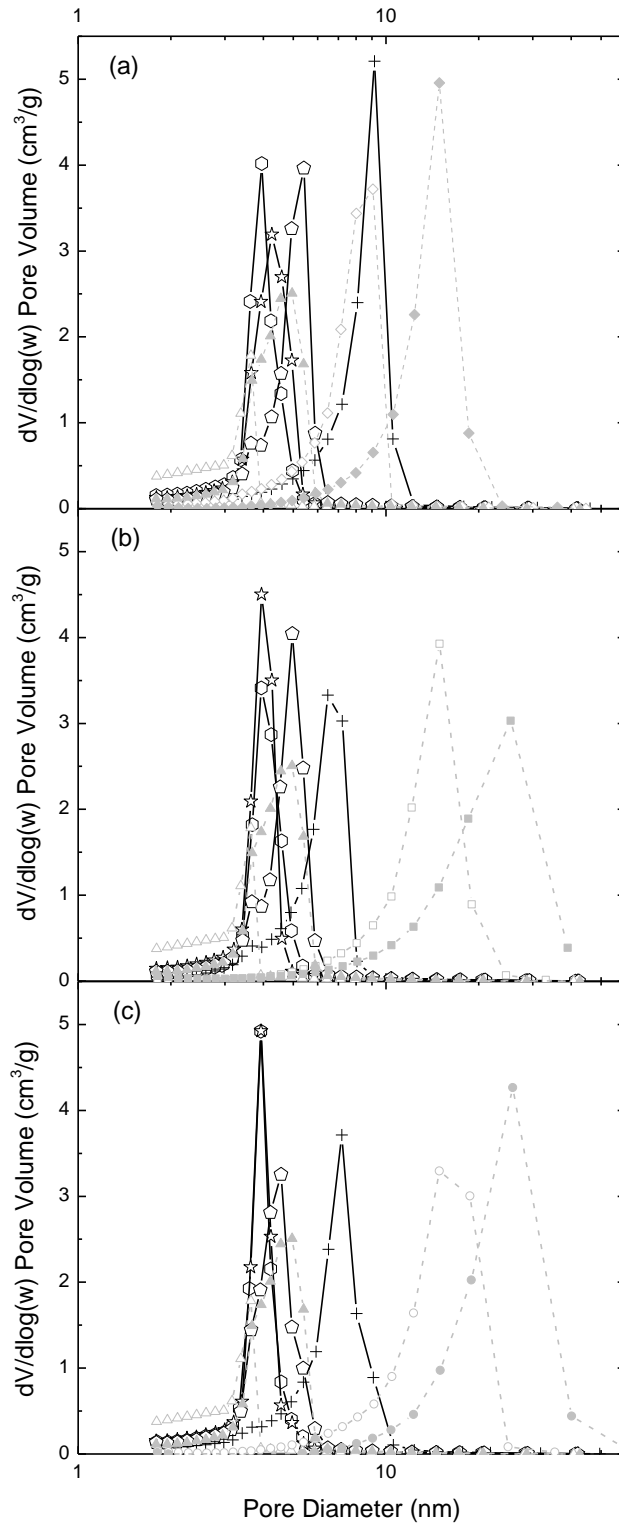
Figure 6. Pore size distributions for (a) \text{Cs}_2\text{CO}_3/\text{Na}_2\text{CO}_3 , (b) \text{CaCO}_3/\text{Na}_2\text{CO}_3 and (c) \text{BaCO}_3/\text{Na}_2\text{CO}_3 at ( \circ ) simultaneous addition, ( \star ) secondary addition at 60%, ( \pentagon ) secondary addition at 70% and ( + ) secondary addition at 80%. Single catalyst data for ( \triangle ) \text{Na}_2\text{CO}_3 , ( \diamond ) \text{Cs}_2\text{CO}_3 , ( \square ) \text{CaCO}_3 and ( \circ ) \text{BaCO}_3 are reproduced for reference (open symbols R/C 100, and closed symbols R/C 200).
