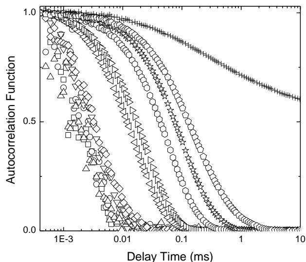
Figure 1. Normalized DLS autocorrelation functions for calcium carbonate at R/C 100. Measurements were taken every 10 % of the total gel time: (□) 0 %, (○) 10 %, (△) 20 %, (▽) 30 %, (◇) 40 %, (◁) 50 %, (▷) 60 %, (◊) 70 %, (☆) 80 %, (⊕) 90 % and (+) 100 %.
