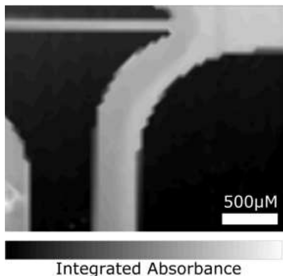
Figure 2: IR absorbance map of mixing zone on chip (point c figure 1)
