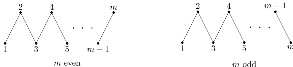
Figure 1: The zigzag poset Z_m .
