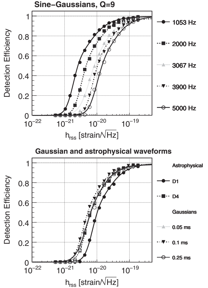
FIG. 5. Software injection efficiency curves for the set of sine-Gaussians of various frequencies (top panel) and Gaussians plus astrophysical waveforms (bottom panel). There is a consistent reduction in efficiency as a function of frequency following the noise distribution.
