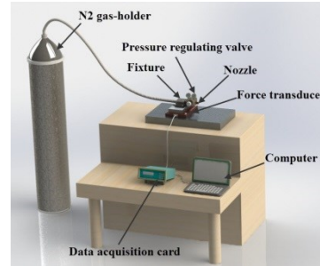
Figure 4 Thrust measuring apparatus
