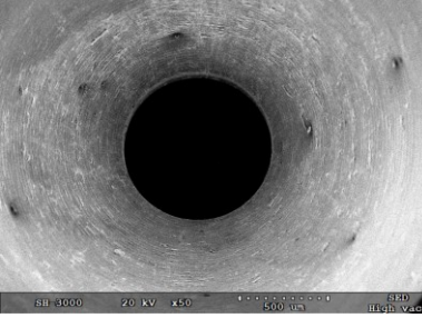
(b) Group B, nozzle machined by ball end mill ( a_p=0.02\text{mm} )
