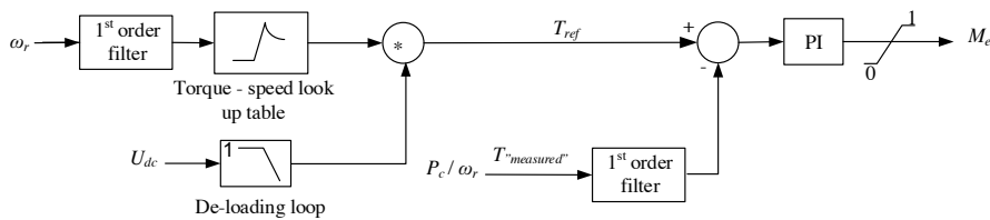
Fig. 4. Block diagram for generator speed controller
