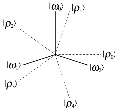
FIG. 2. The optimal POVM directions (thick solid lines) given by theorem 2 in the case of M = 5 . The input states are represented as (-1)^k |\psi_k\rangle by the dashed lines whose lengths correspond to a unit state vector. The lengths of the thick solid lines are scaled according to the normalization factors of the corresponding POVM elements.
