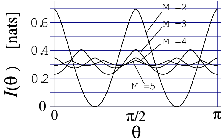
FIG. 1. The Shannon mutual information I(\theta) in nats versus the optimization parameter \theta for M=2, 3, 4 and 5 .
