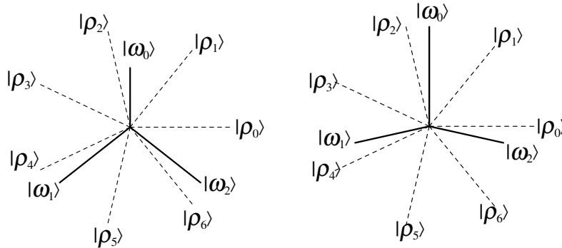
FIG. 3. The two inequivalent optimal POVMs in the case of M = 7 . The POVM directions and input states are represented by thick and dashed lines respectively according to the conventions of Fig. 2.
