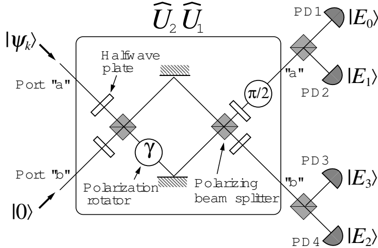
FIG. 4. The optical circuit implementing \mathcal{W} = \{\hat{\omega}_0^*, \hat{\omega}_1^*, \hat{\omega}_2^*\} . It consists of the unitary transformation \hat{U}_2\hat{U}_1 followed by the measurement \{|E_j\rangle\} . \hat{U}_2\hat{U}_1 is effected by four halfwave plates, two polarizing beam splitters, and two polarization rotators. The measurement \{|E_j\rangle\} is made by photon counting at the four output ports.
