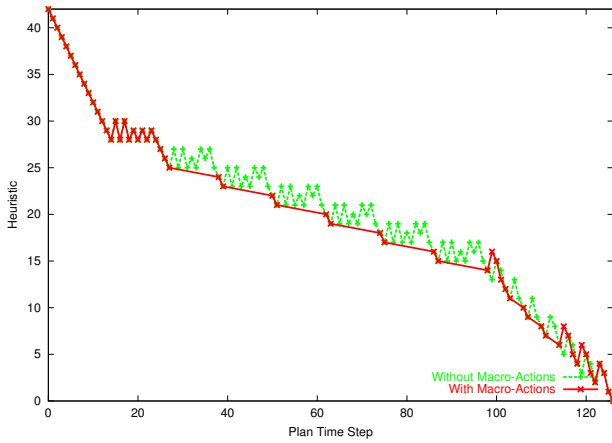
Figure 1: Heuristic Landscape over Makespan, With and Without Macro-Actions
