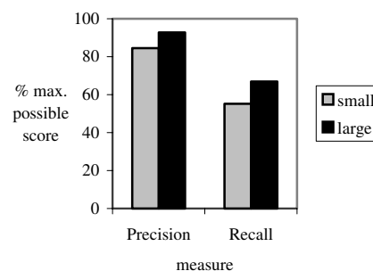
Figure 6. Percentage of the maximum possible precision and recall scores achieved in many-to-one mappings
