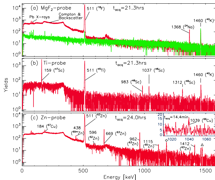
Figure 4. Activation spectra of the \text{MgF}_2 (a), Ti (b) and Zn targets (c) derived in this work. Energies of the most prominent transitions are labeled in conjunction with their assigned photo-nuclear reaction product given in brackets. The raw \text{MgF}_2 activation spectra are shown in red color in (a) together with the natural background radiation which was measured for the same \Delta t_{\text{acq}} after the \text{MgF}_2 target and the Ta radiator were removed (green). The dominating 511 keV annihilation peak results from the \beta^+ decay of ^{18}\text{F} . The background-corrected titanium activation spectra are depicted in (b). The most prominent peak at 159 keV is caused by ^{48}\text{Ti}(\gamma, p)^{47}\text{Sc} and the subsequent decay of ^{47}\text{Sc} . The three transitions at 983, 1037 and 1312 keV belong to the decay of ^{48}\text{Sc} , produced via ^{49}\text{Ti}(\gamma, p)^{48}\text{Sc} . The activation spectra for the natural Zn sample ( \Delta t_{\text{acq}} = 24.0 h) are shown in (c). The intense 511 keV photopeak corresponds to annihilation following the \beta^+ decay of ^{63}\text{Zn} . Summation peaks of the strongest photopeaks are also seen (511 + 669 keV ( \diamond ), 511 + 962 keV ( \Delta )). The inset in the picture (blue) shows the presence of the 1039 keV transition resulting from the fast decay of ^{66}\text{Cu} ( t_{1/2}^{\text{Lit.}} = 5.12 min) emerging from ^{67}\text{Zn}(\gamma, p)^{66}\text{Cu} as observed for \Delta t_{\text{acq}} = 14.40 min. All spectra show the 1460 keV background radiation associated with ^{40}\text{K} .
