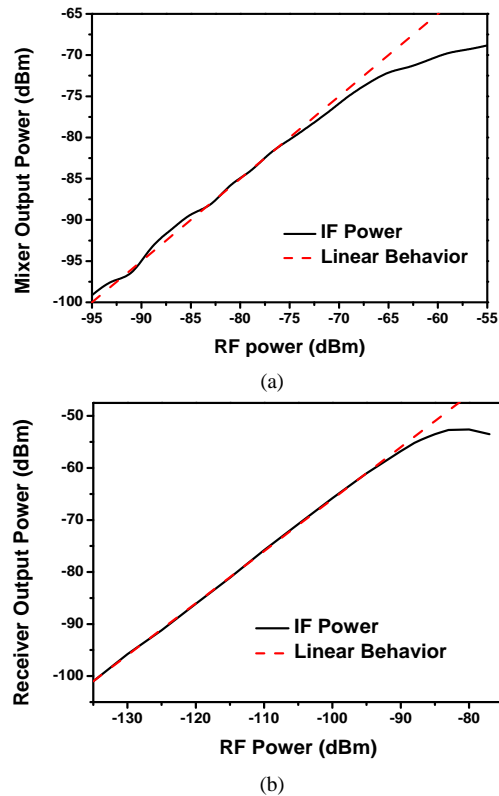
Fig. 9. (a) Simulated IF output power versus RF input power, and (b) its measurement result.
