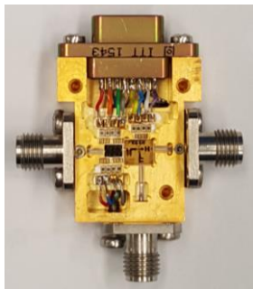
Fig.5. Photograph of packaged HTS receiver front-end module.
