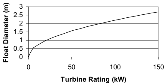
Figure 6: Float diameter versus turbine rating (maximum tidal velocity = 2.5\text{ms}^{-1} ).
