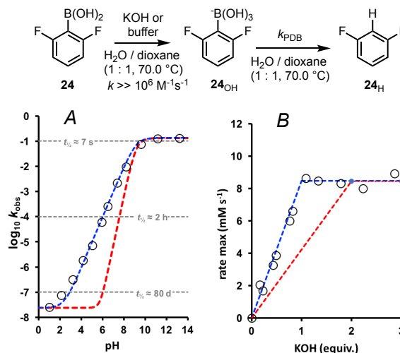
Figure 1. Protodeboronation of 2,6-difluorophenyl boronic acid ( 24 , 51 mM), 70 °C. Circles experimental data. Graph A: pH- \log k_{obs} profile; buffered pH. Blue line: mono-anionic mechanisms (e.g. I/II/IV) where k_{obs} = k_{PDB}/\{1+10^{(pK_a-pH)}\} + k_b ; pK_a = 9.15 , k_{PDB} = 0.135 \text{ s}^{-1} , and k_b = 3 \times 10^{-8} \text{ s}^{-1} . The latter is a very slow uncatalyzed process. 14e,14m Red line: mechanism III where ( k_{obs} = k'_{III}(10^{(pH-pK_w)})/\{1+10^{(pK_a-pH)}\} + k_b ); pK_a = pK_{III} ; k'_{III} = 0.135 \text{ s}^{-1} ; k_b = 3 \times 10^{-8} \text{ s}^{-1} . Graph B: rate dependence on KOH stoichiometry.
