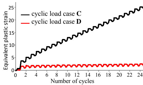
Fig. 7 Abaqus verification of the ratchet limit for the cyclic temperature of \Delta\theta = 200^\circ C using detailed step by step analysis
