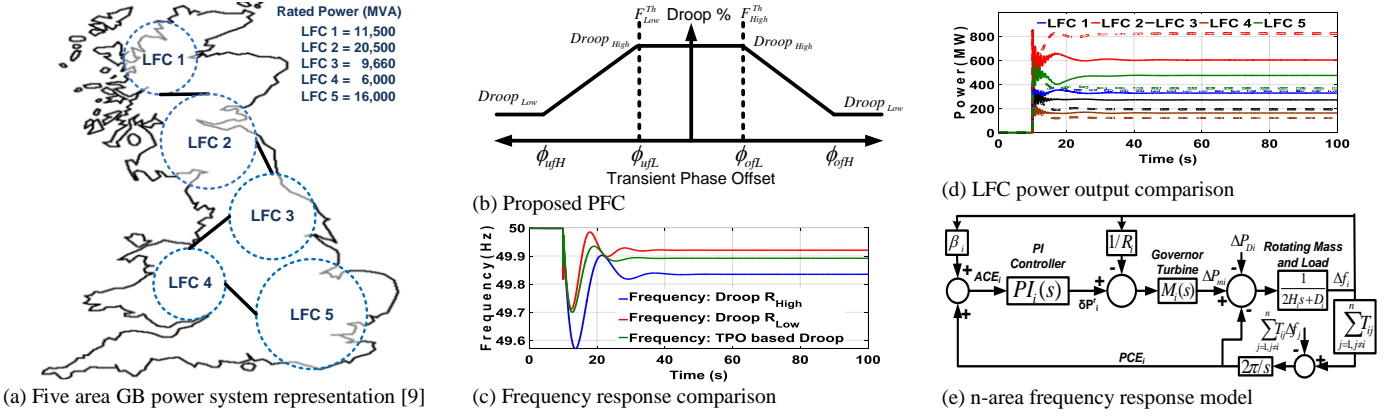
(a) Five area GB power system representation [9] (b) Proposed PFC (c) Frequency response comparison (d) LFC power output comparison (e) n-area frequency response model Fig. 2. Power system representation, proposed droop curve, system response to 1850 MW generation loss and n-area frequency response model.
