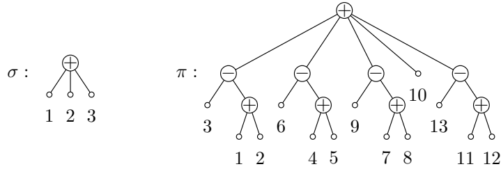
FIGURE 1. The separating trees of two permutations \sigma and \pi
