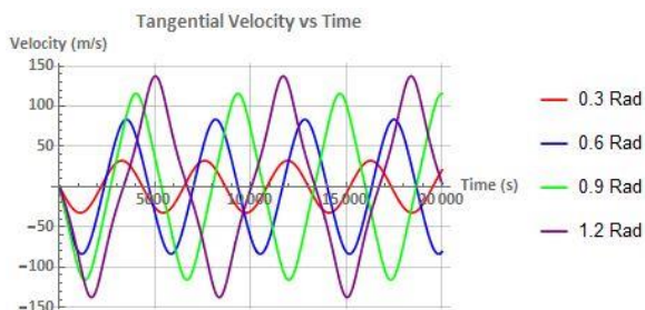
Fig. 24. An example of the tangential velocity vs time chart for a tether system.
