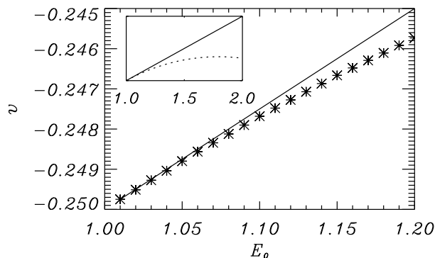
FIG. 3: Analytical velocity given by Eq. (7) (continuous line) compared with numerical results (symbols) from the original model (1). In the inserted plot we compare the velocities far from threshold. Same parameters of Fig. 1.
