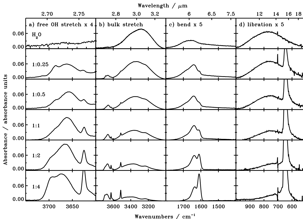
Fig. 2. Spectra over the 4000–400 \text{cm}^{-1} range at 15 K of the four H 2 O peaks in H 2 O:CO 2 1:x ice mixtures for different CO 2 concentrations. Each column contains one of the H 2 O modes and each row one of the H 2 O:CO 2 mixtures: a) an expanded view of the H 2 O free OH stretch, b) the H 2 O bulk and free-OH stretch, c) the H 2 O bend and d) H 2 O libration. The intensities of the libration, bend and free-OH stretch bands have been scaled, with a scaling factor indicated in the first row. The H 2 O exposure was kept constant in all experiments. The narrow peaks around 3500 and 3630 \text{cm}^{-1} have been previously assigned to CO 2 combination modes (Sandford & Allamandola 1990). The sharp feature around 700 \text{cm}^{-1} is an experimental artifact.
