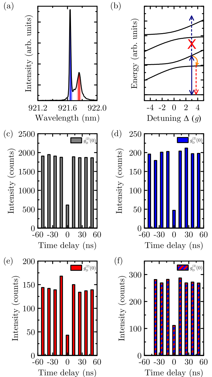
FIG. 4. Photon-blockade regime: (a) Spectrum of the strongly coupled system at \Delta = 3.5g and resonant excitation of UP1 with an 80 ps long pulse. The emission from UP1 is illustrated in blue on the left and the emission from LP1 in red on the right. (b) Illustration of the JC-ladder. The excitation laser is resonant with UP1 (depicted with a solid blue upward arrow) but not resonant with higher climbs up the ladder. Following excitation of UP1, possible recombination channels are from UP1 to the ground state (solid blue downward arrow) or from LP1 to the ground state (dashed red arrow) via a phonon-assisted population transfer from UP1 to LP1 (curved orange arrow). (c-f) Correlation measurement of the (c) unfiltered signal, revealing g_D^{(2)}(0) = 0.330 \pm 0.003 , (d) filtered emission from UP1, revealing g_D^{(2)}(0) = 0.227 \pm 0.008 , (e) filtered emission from LP1, revealing g_D^{(2)}(0) = 0.284 \pm 0.011 and (f) cross-correlation between UP1 and LP1, revealing g_D^{(2)}(0) = 0.405 \pm 0.005 .
