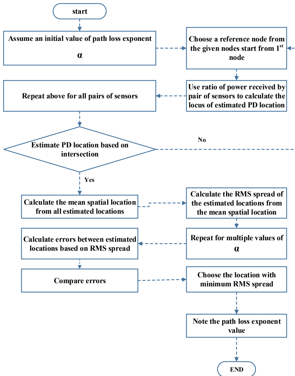
Figure 2. Algorithm flowchart.
