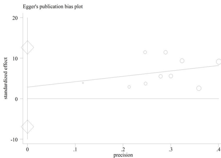
Figure 4: Publication bias
