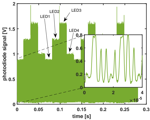
Fig. 3. Received signal of the photodiode at a data rate of 0.9 Mb/s. The main plot shows a time scale of several camera frames, indicating the times during which different LEDs are transmitting. The inset shows a time scale of several transmitted bits.
