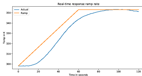
Figure 1 Real-time response to ramp rate of heater mat.
