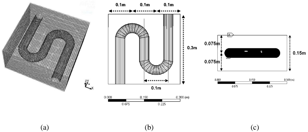
8 Figure 8: Validation configuration of (a) meshing technique (b) plan dimension (c) depth dimension 9
