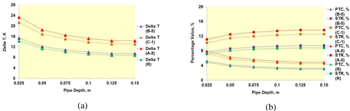
12 Figure 12: RPSC performance based on pipe depth in (a) Delta T (b) PTC and STR
