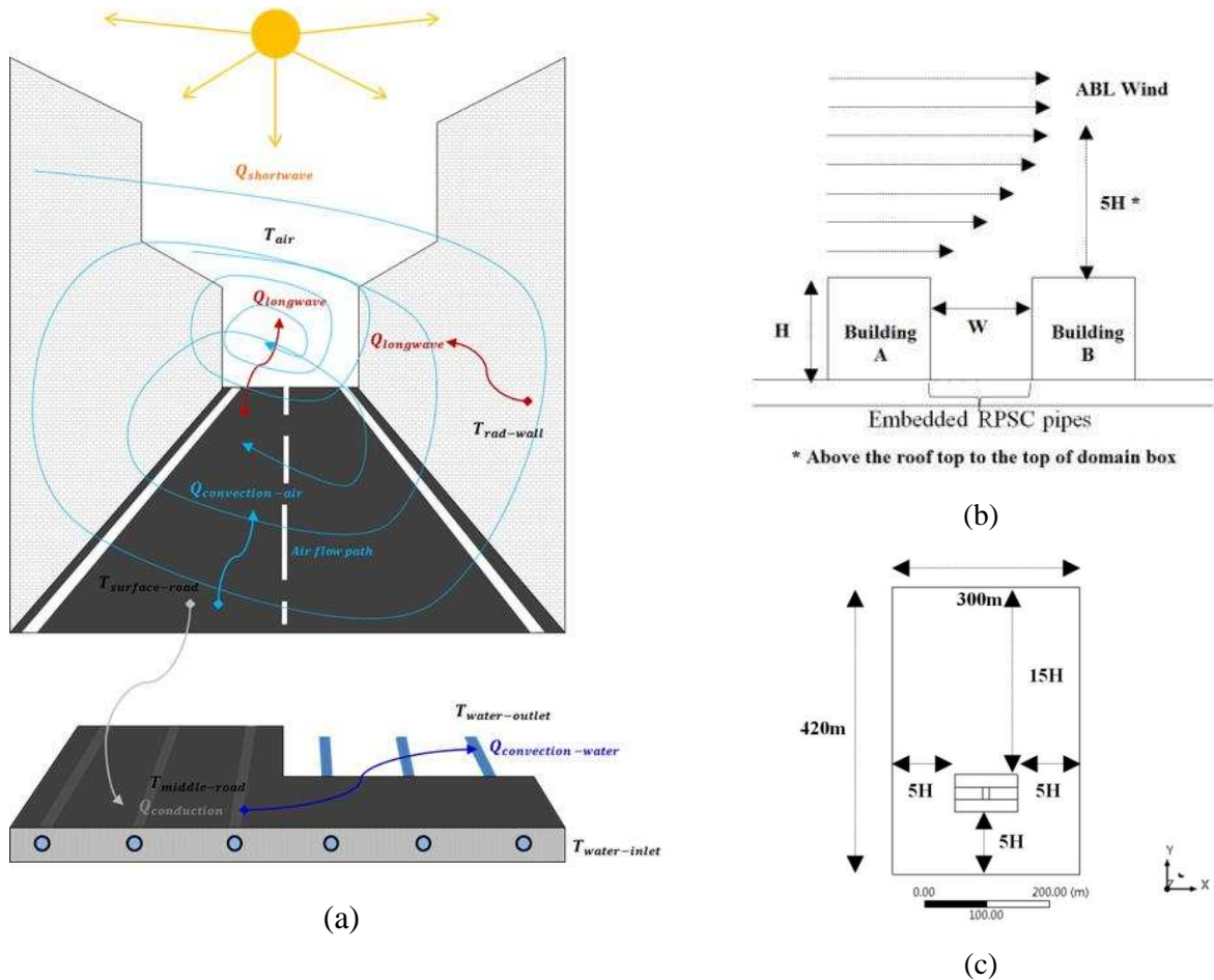
1 Figure 2: Urban domain (a) in 3-dimensional diagram (b) from elevation view (c) from top view
