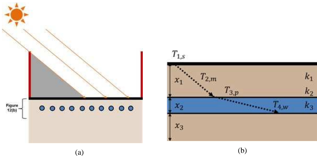
23 Figure 4: Diagram of heat transfer of (a) external to surface micro domain (b) surface to internal
