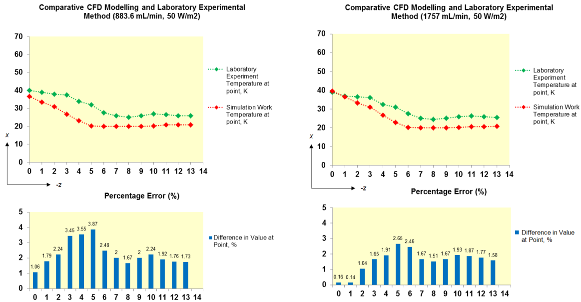
1 Figure 10: Trend comparison between the current simulation and the experimental results according 2 to the depth from the surface of (a) 883.6 mL/min (b) 1757 mL/min
