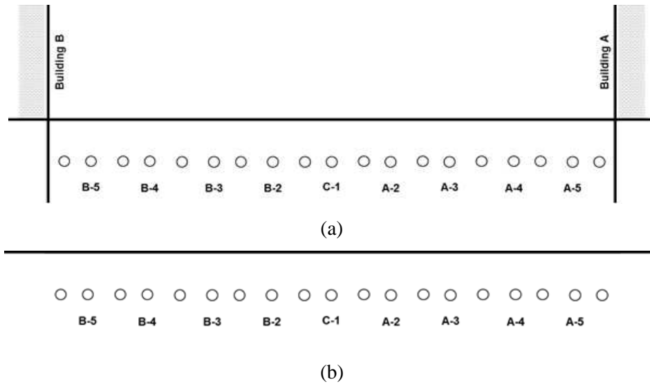
4 Figure 3: Embedment of RPSC pipes in (a) urban model (b) flat/rural model (Not to Scale)
