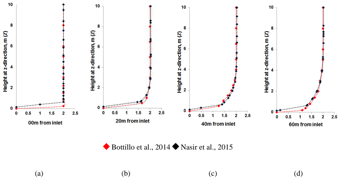
14 Figure 5: Validation of wind velocity at four locations based on y-direction
